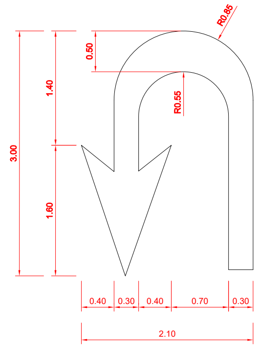
DETAIL - 03: U-TURN MARKING ARROW DETAIL N.T.S
